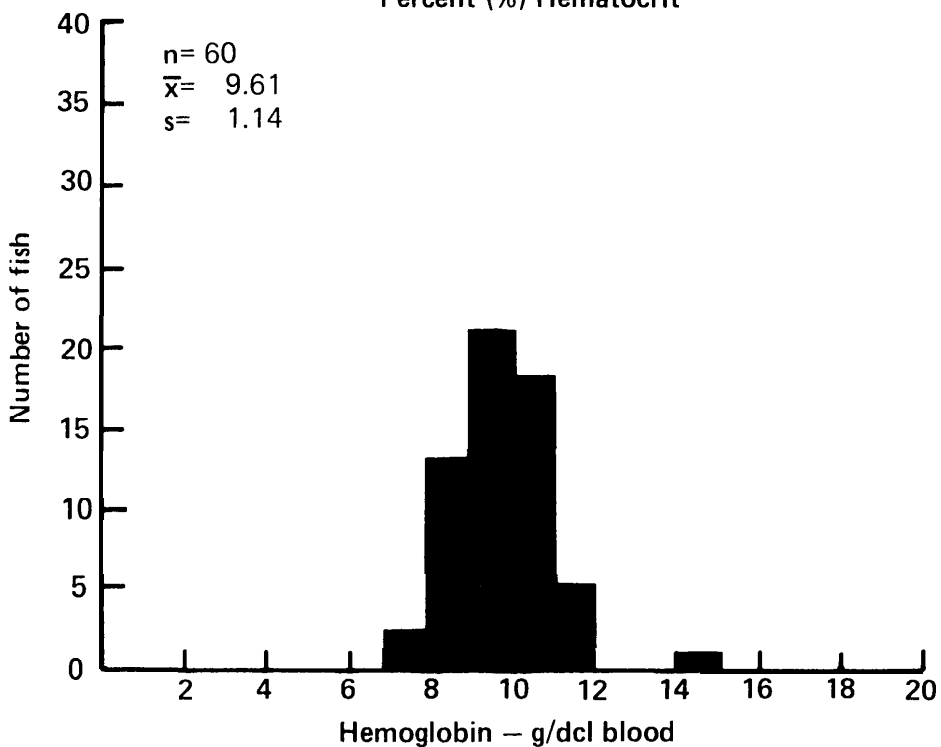
Figure 4. --Frequency histogram for hematocrit and hemoglobin values for the Wells (Winthrop) Hatchery steelhead in 1979. Number of fish sampled ( n ), mean hemoglobin and hematocrit values ( \bar{x} ), and standard deviations ( s ) are also given.
